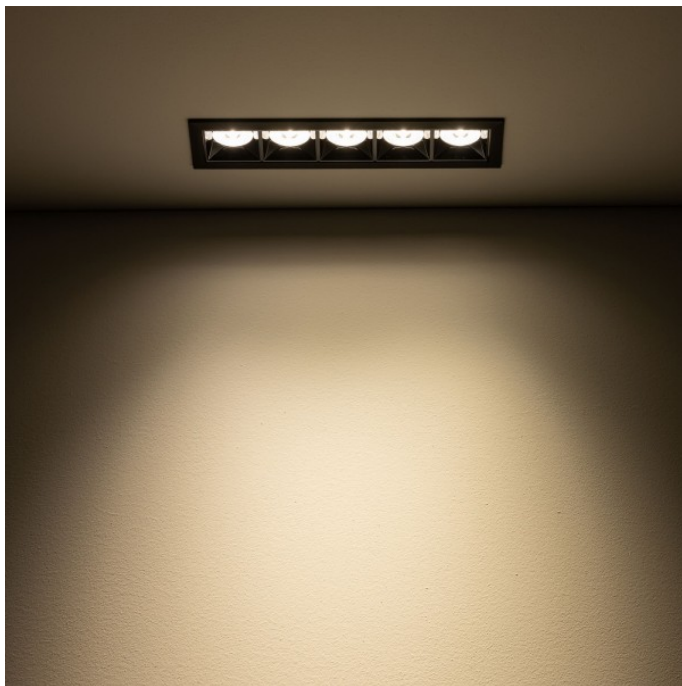
MIDI LED BLACK 20W 3000K RECESSED 10062 Nowodvorski
